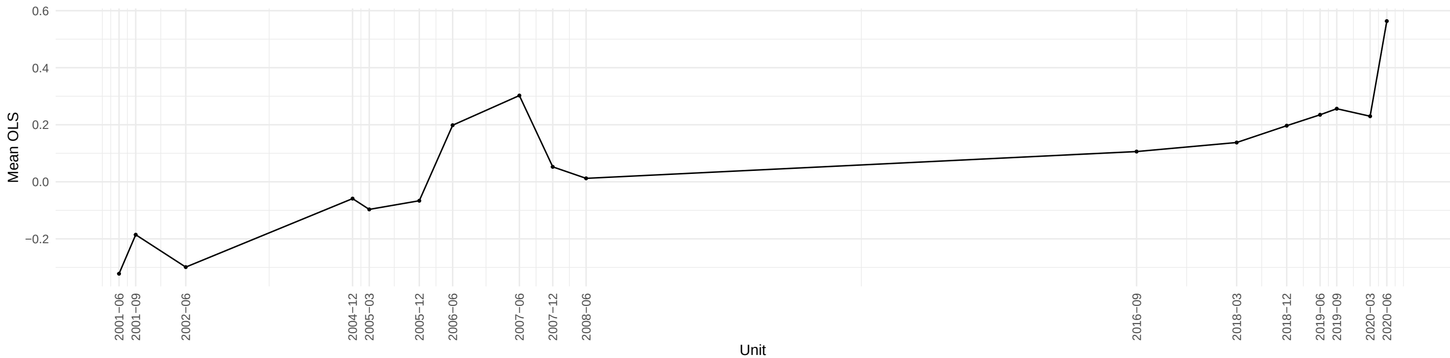
Evolution of T5YFFM OLS coefficient across time
