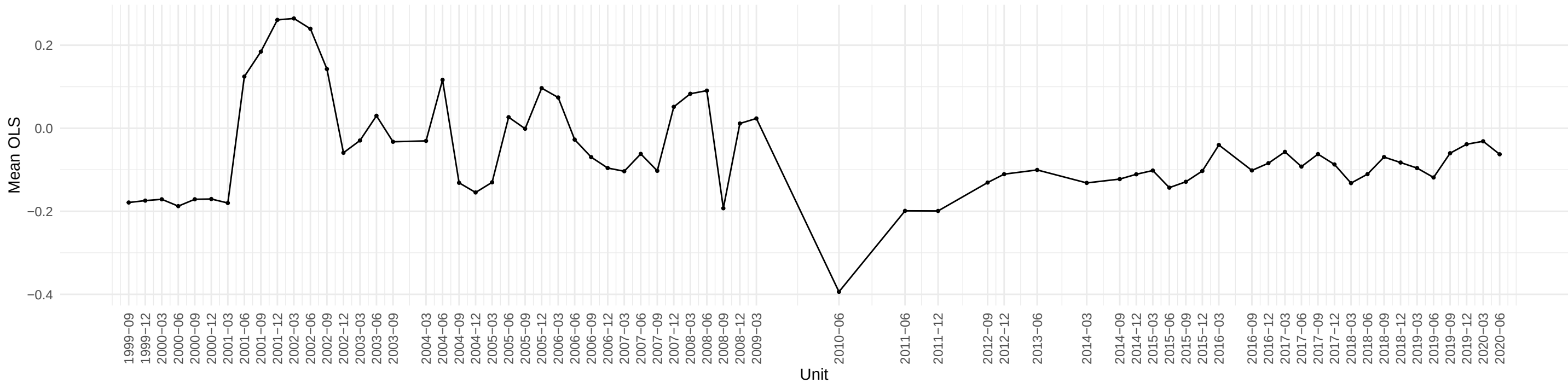
Evolution of TB6MS OLS coefficient across time
