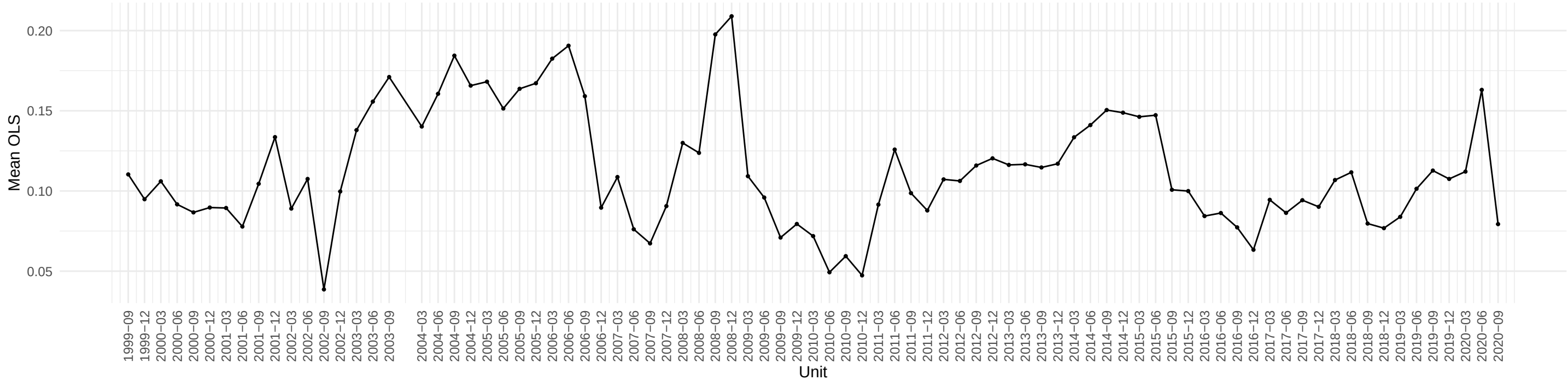
Evolution of UEMP15OV OLS coefficient across time
