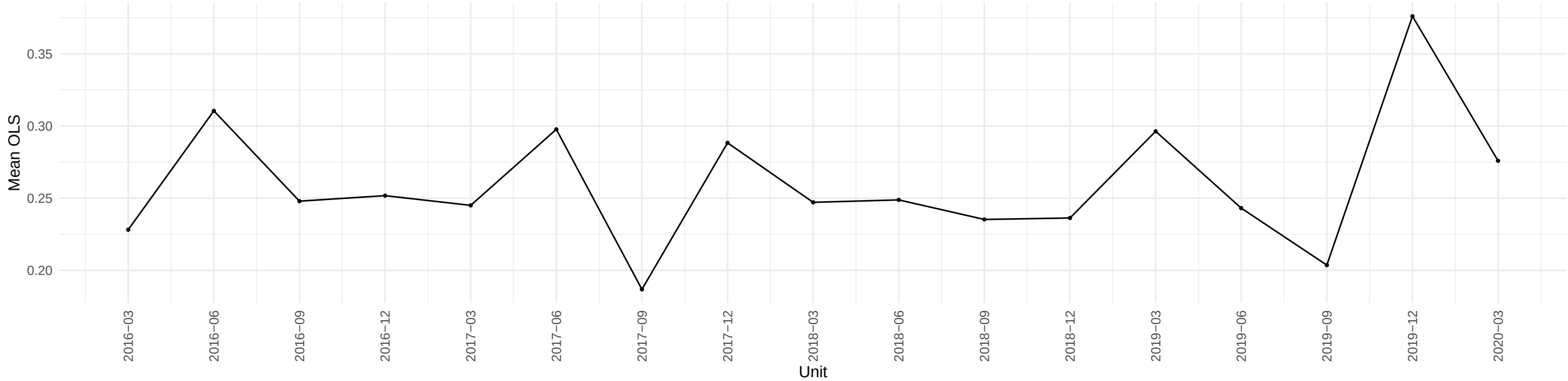
Evolution of WPSID61 OLS coefficient across time
