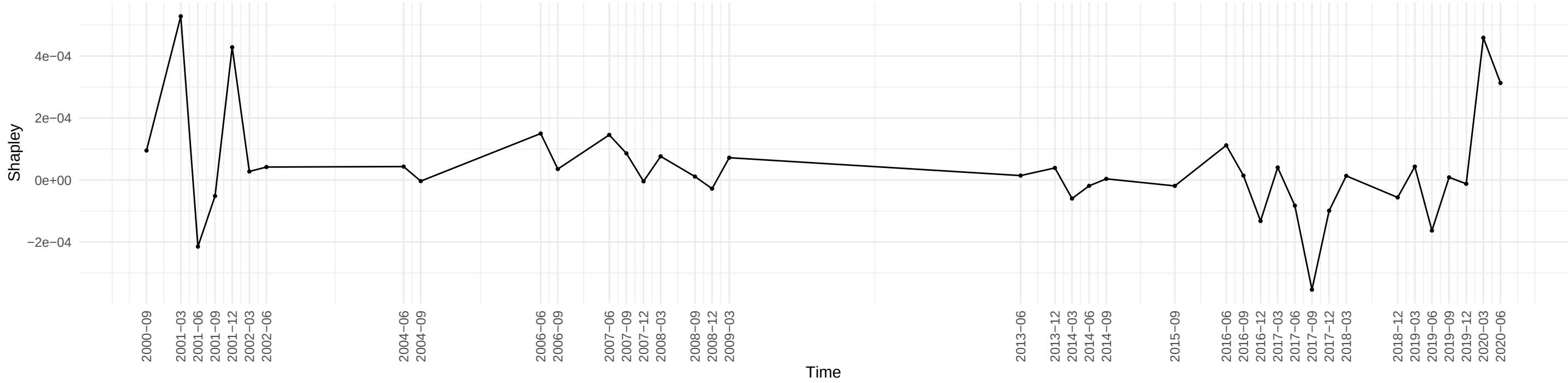
Evolution of Shapley Value of ANDENOX across time
