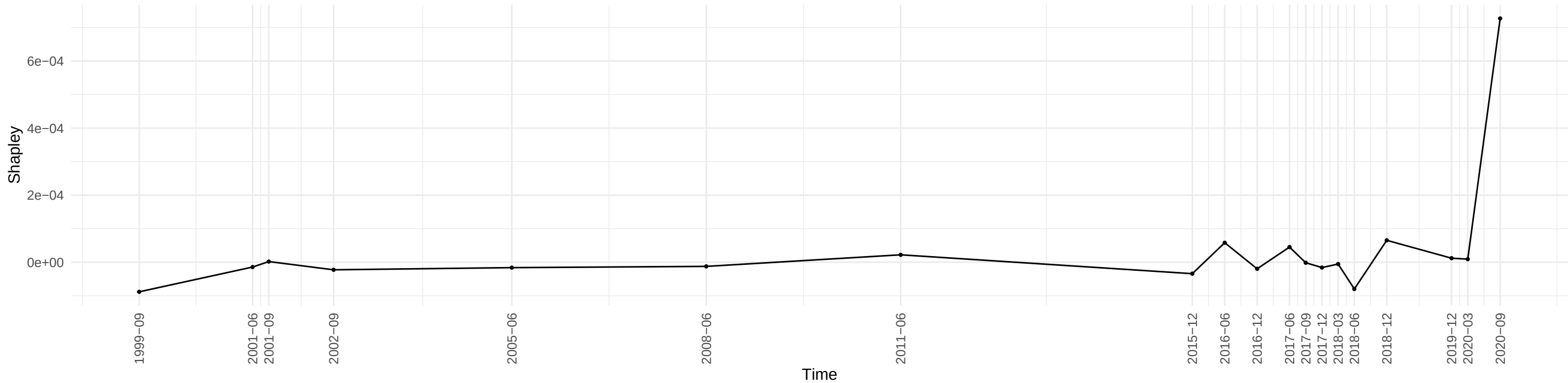
Evolution of Shapley Value of BUSLOANS across time
