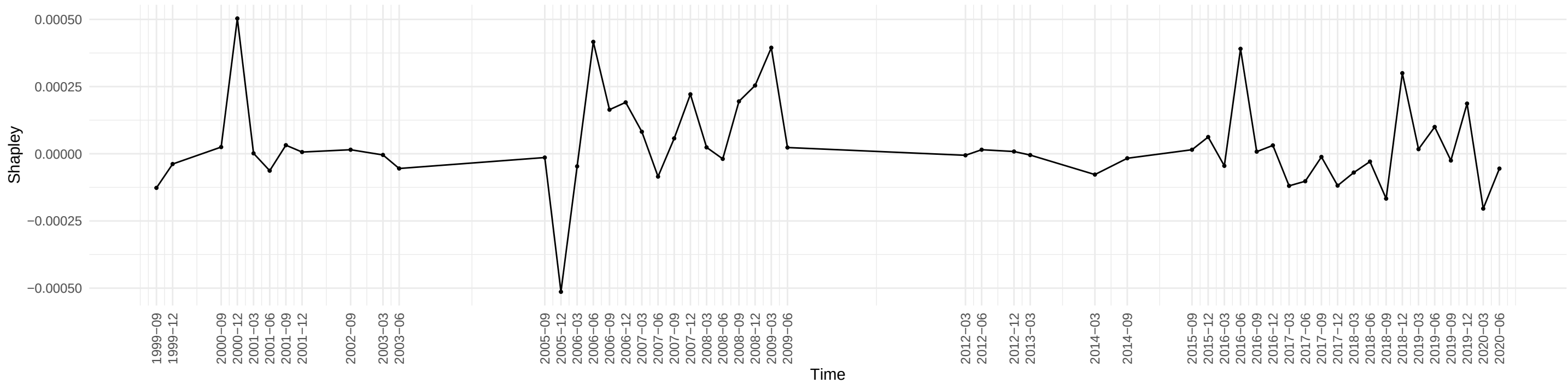
Evolution of Shapley Value of CLAIMSx across time
