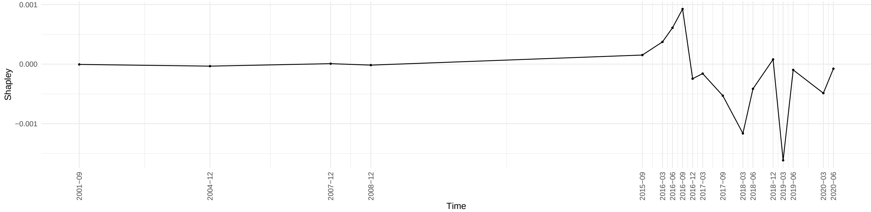
Evolution of Shapley Value of CPIMEDSL across time
