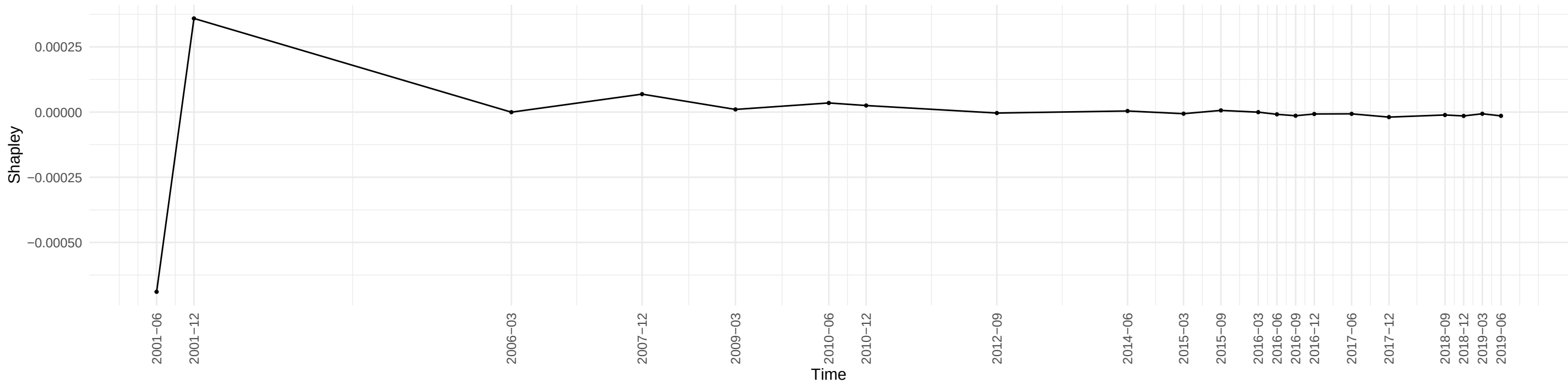
Evolution of Shapley Value of DNDGRG3M086SBEA across time
