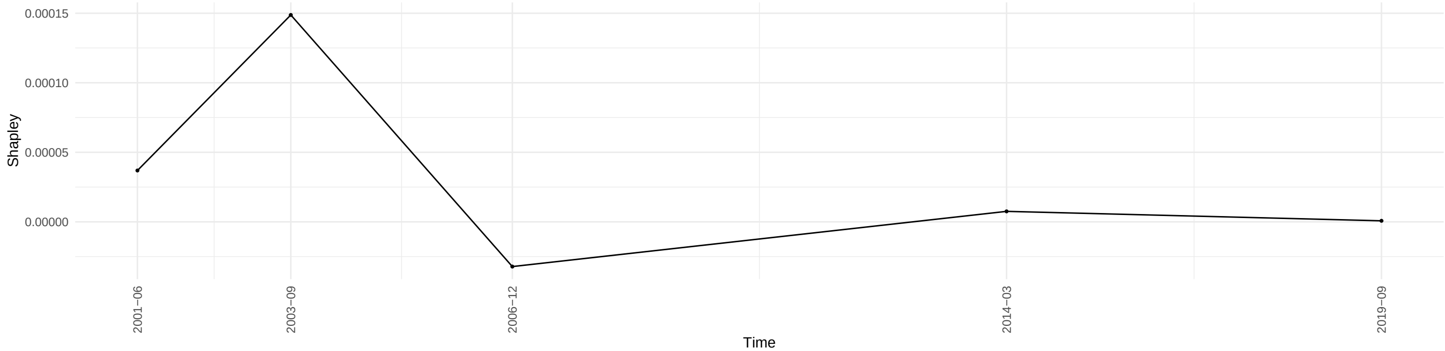
Evolution of Shapley Value of DTCTHFNM across time
