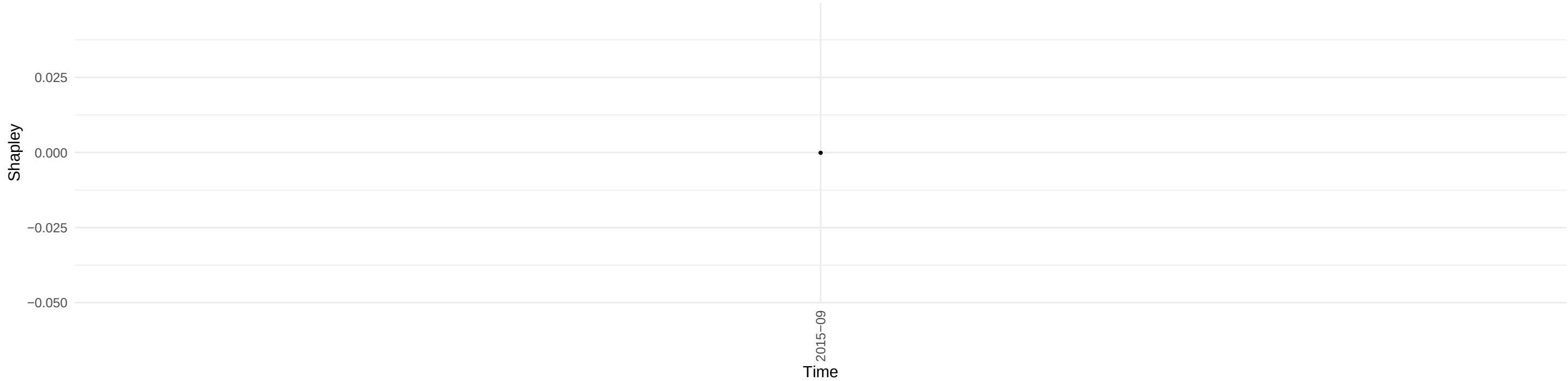
Evolution of Shapley Value of NAPMPRI across time
