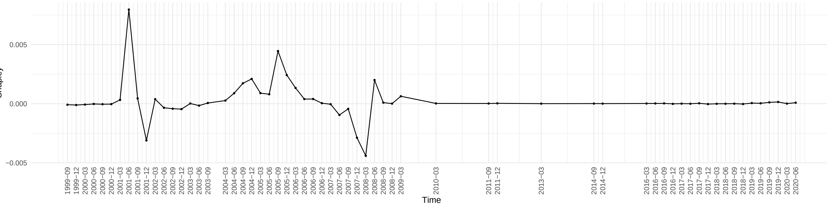
Evolution of Shapley Value of TB3MS across time
