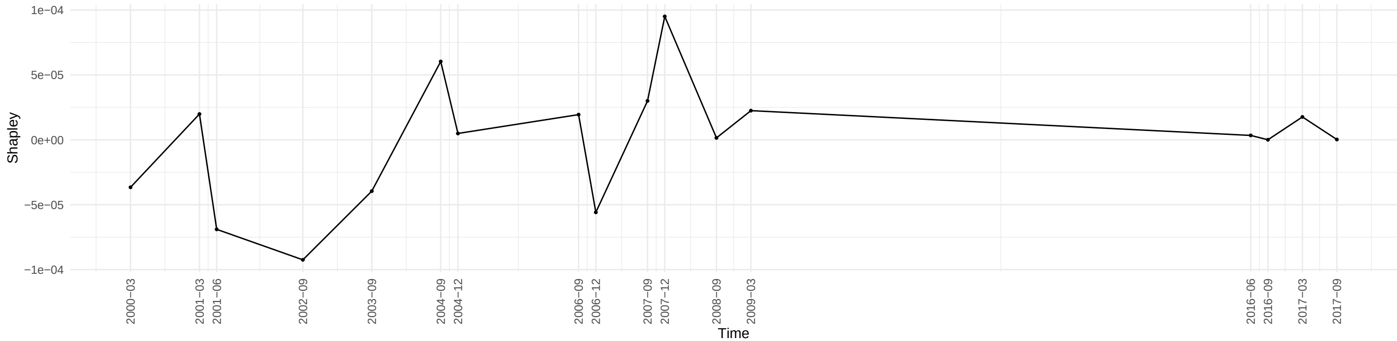
Evolution of Shapley Value of UEMPMEAN across time
