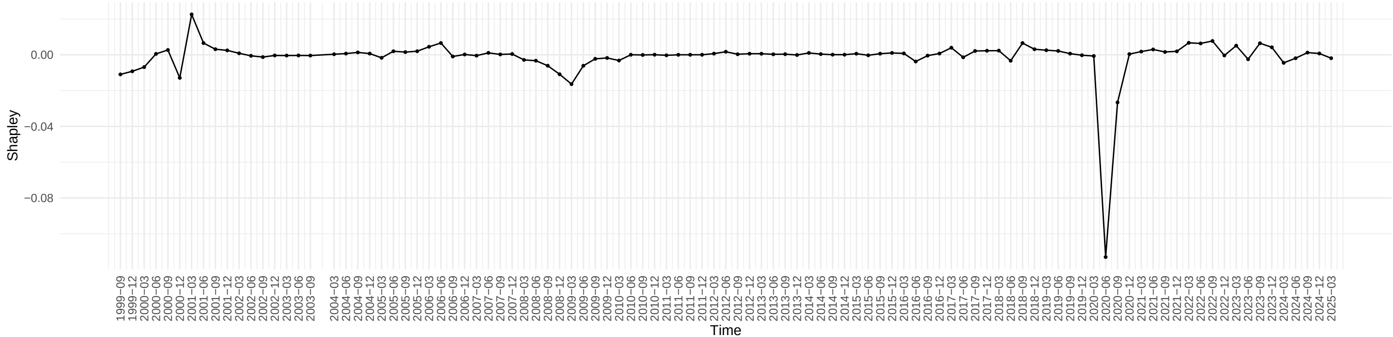
Evolution of Shapley Value of USWTRADE across time
