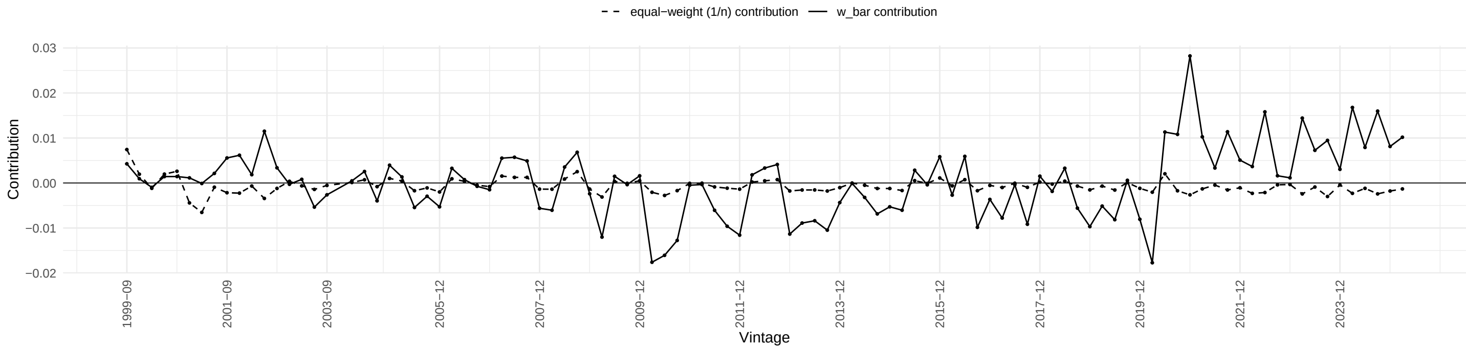
CES3000000008 – w_bar vs equal-weight contribution
