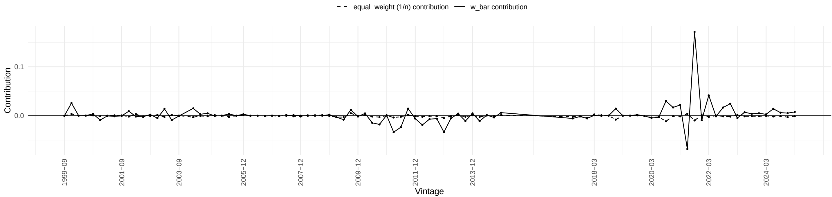
CUSR0000SAD – w_bar vs equal-weight contribution
