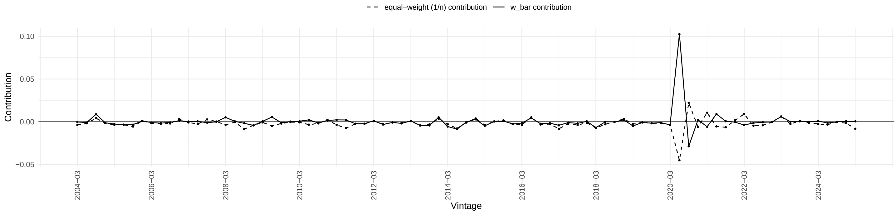
DPCERA3M086SBEA – w_{\text{bar}} vs equal-weight contribution
