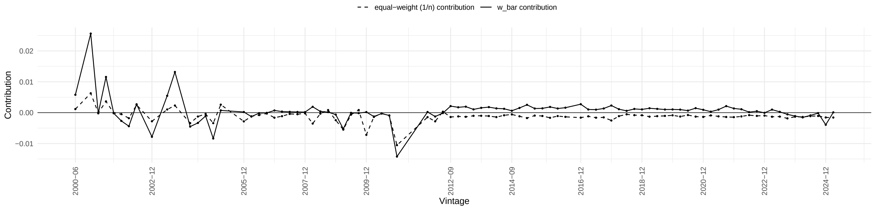
DTCTHFNM – w_{\text{bar}} vs equal-weight contribution
