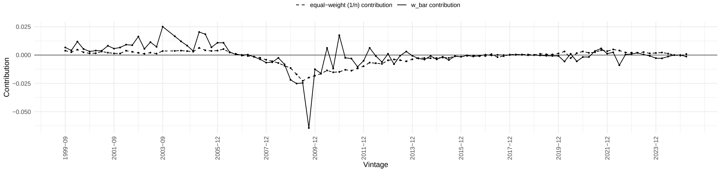
HOUSTS – w_{\text{bar}} vs equal-weight contribution
