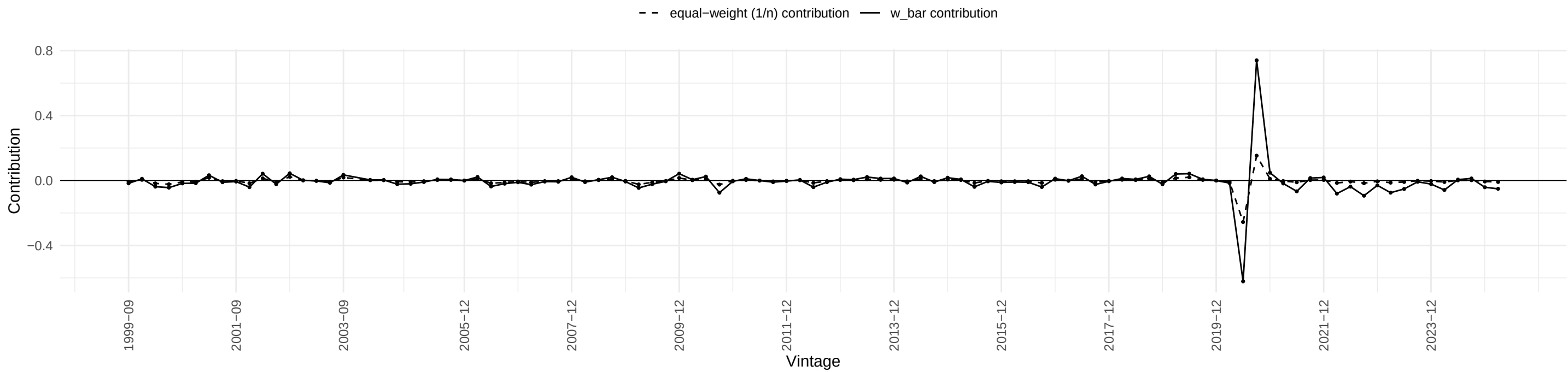
UEMP5TO14 – \bar{w} vs equal-weight contribution
