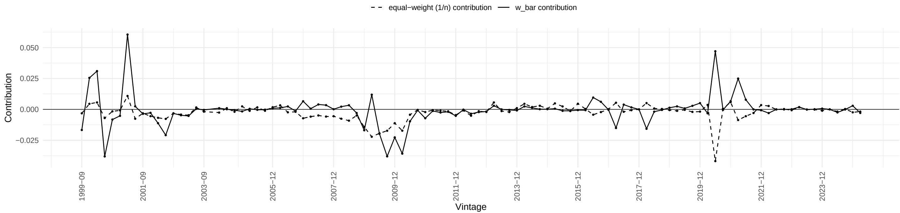
USCONS – w_bar vs equal-weight contribution
