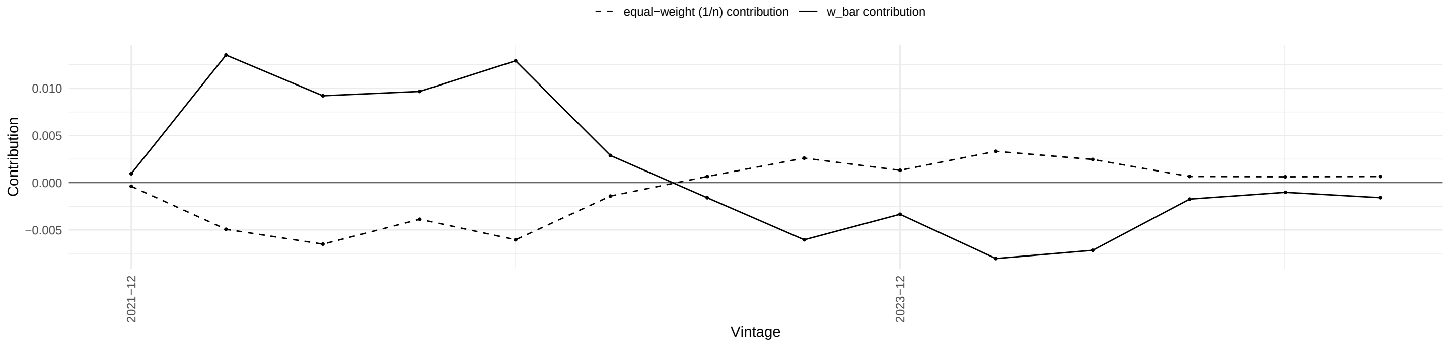
VIXCLSx – w_{\text{bar}} vs equal-weight contribution
