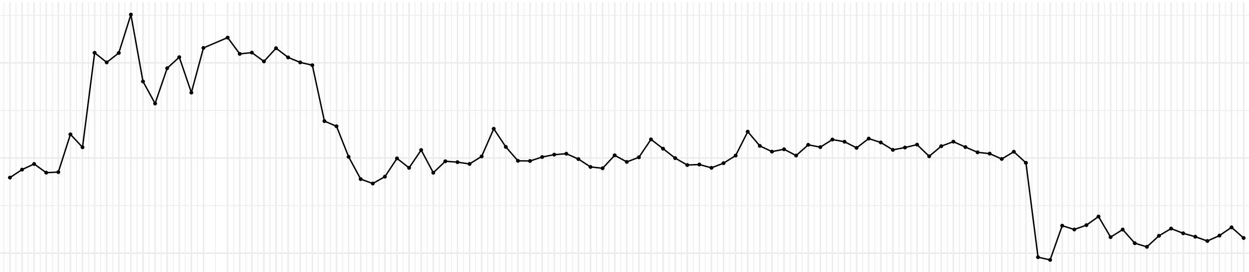
Evolution of AMDMUOx OLS coefficient across time
