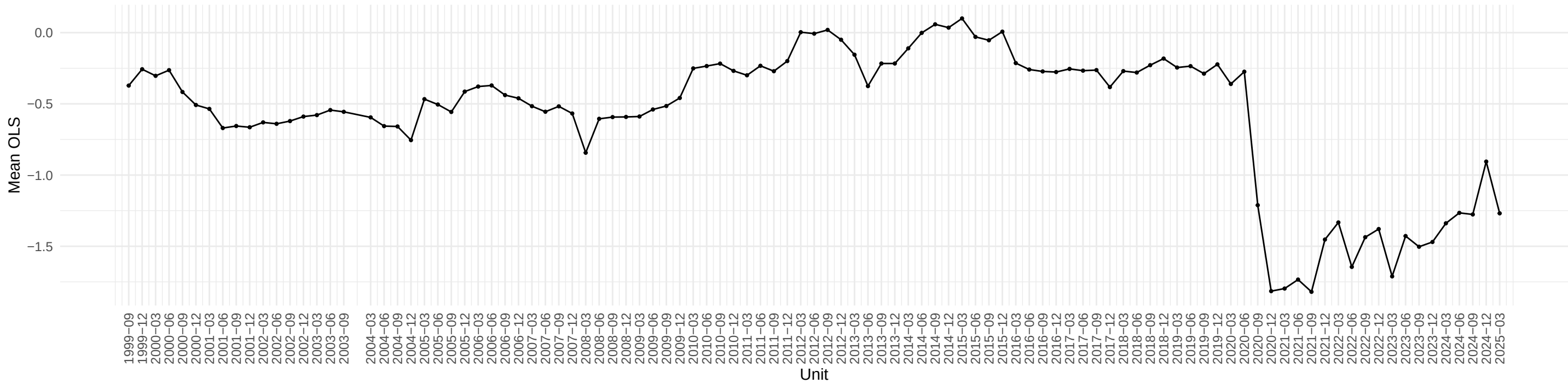
Evolution of CES3000000008 OLS coefficient across time
