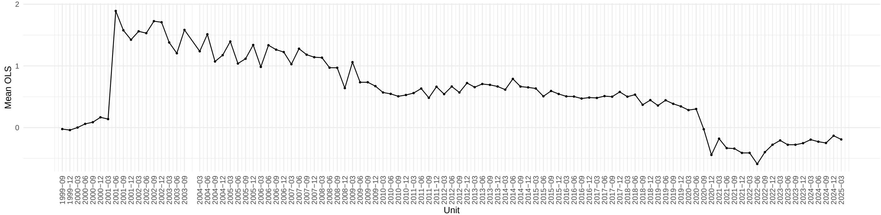
Evolution of COMPAPFFx OLS coefficient across time
