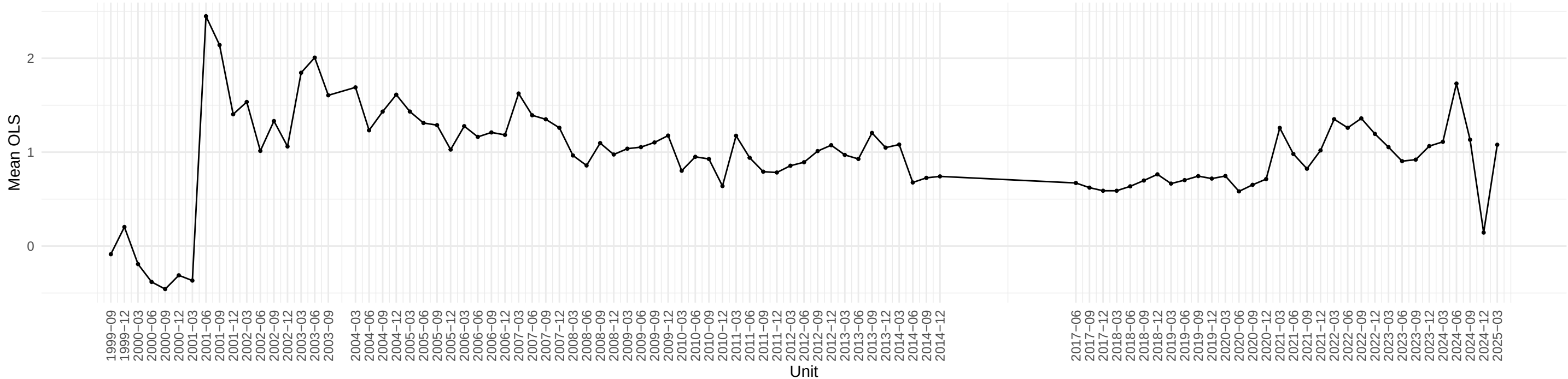
Evolution of CUSR0000SA0L2 OLS coefficient across time
