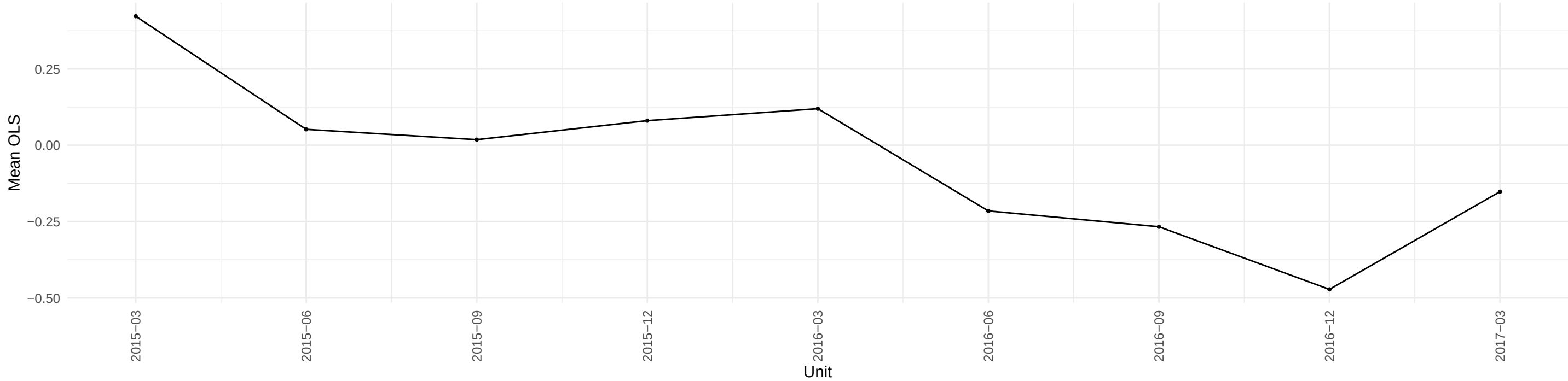
Evolution of CUUR0000SAD OLS coefficient across time
