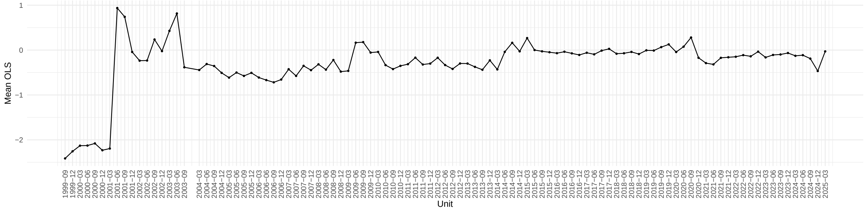
Evolution of EXCAUSx OLS coefficient across time
