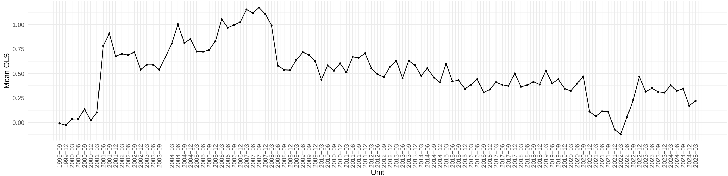
Evolution of EXJPUSx OLS coefficient across time
