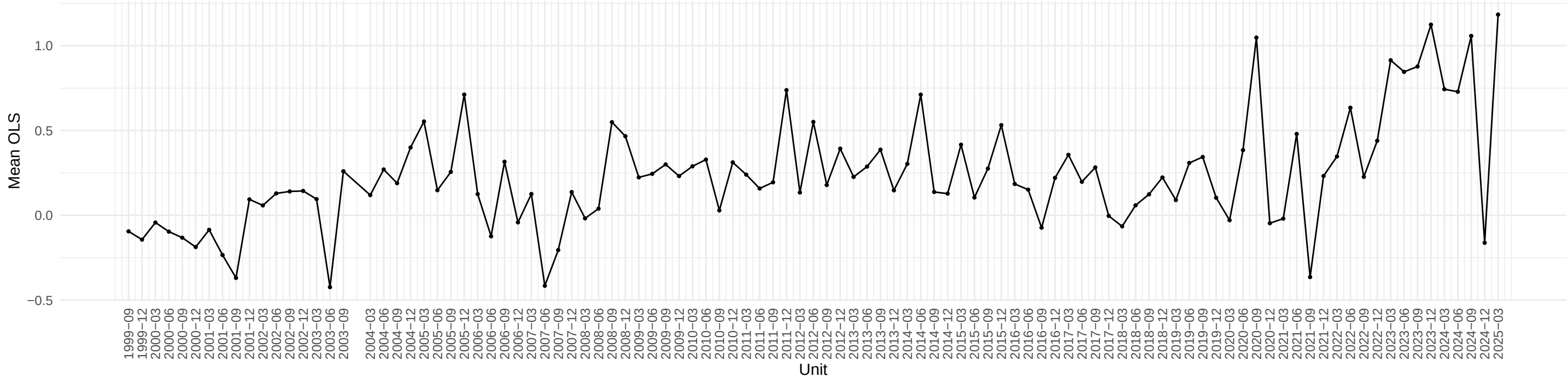
Evolution of FEDFUNDS OLS coefficient across time
