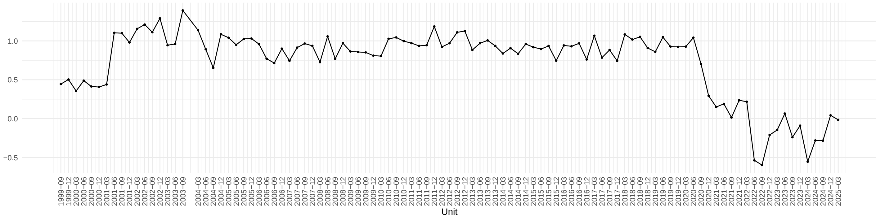
Evolution of GS1 OLS coefficient across time
