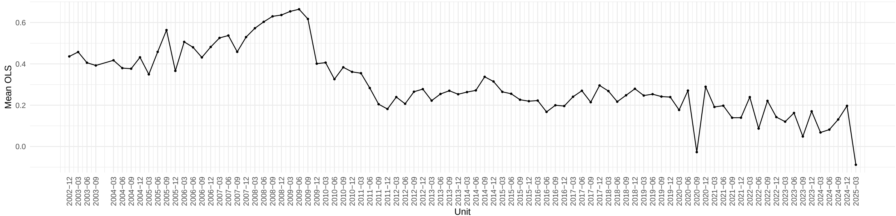
Evolution of IPDCONGD OLS coefficient across time
