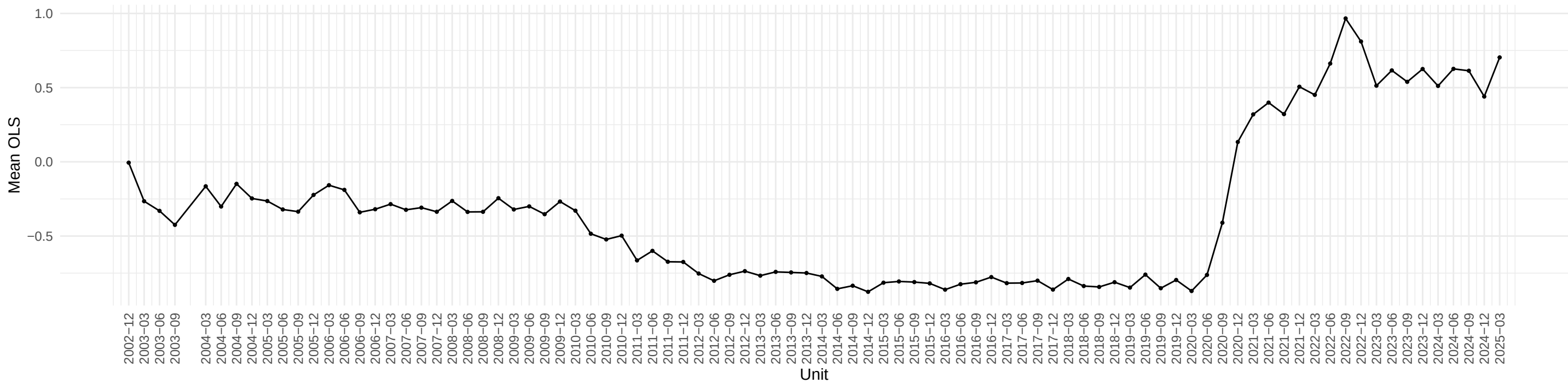
Evolution of IPFUELS OLS coefficient across time
