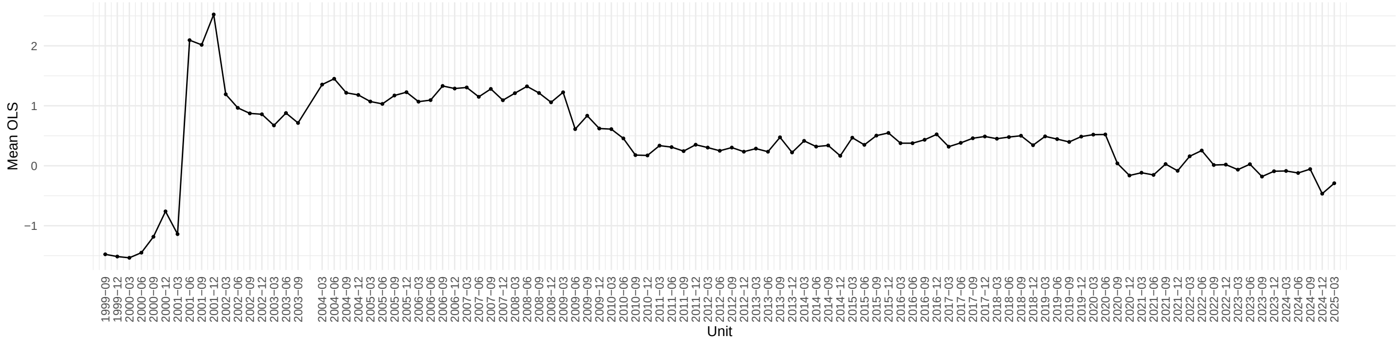
Evolution of M2SL OLS coefficient across time
