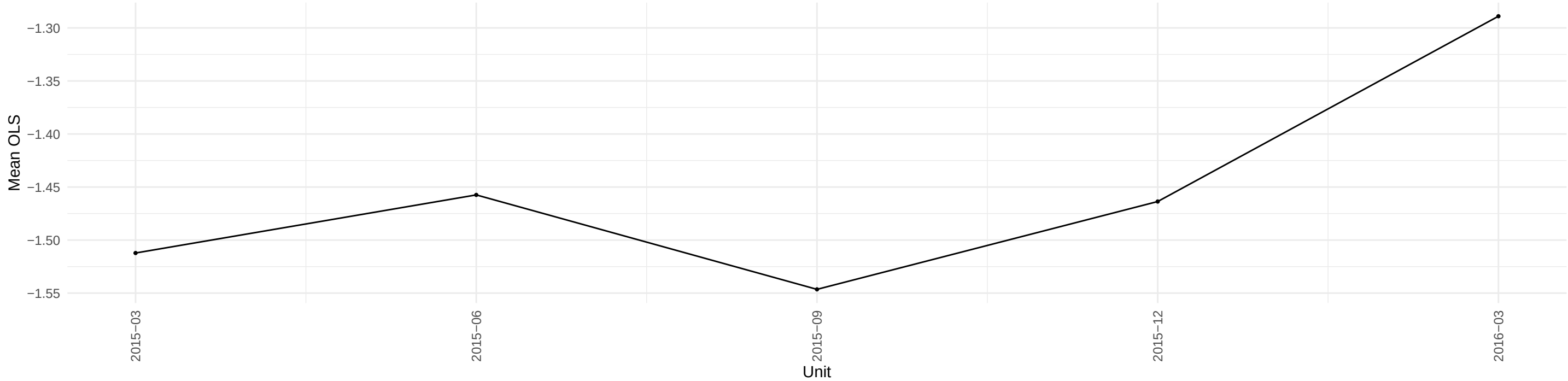
Evolution of NAPMPRI OLS coefficient across time
