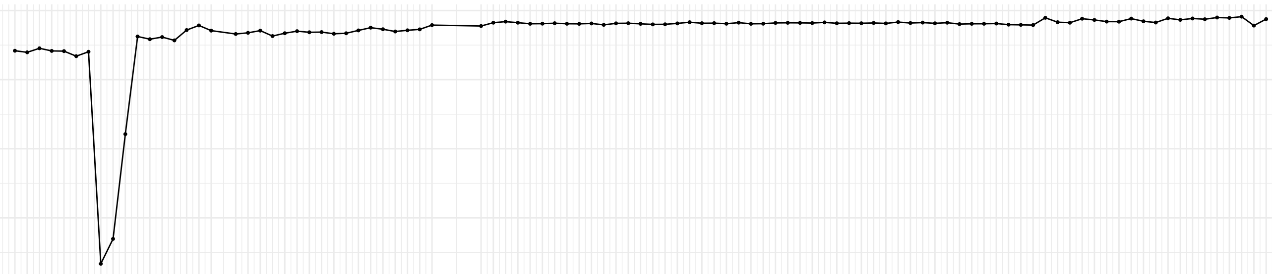
Evolution of NONBORRES OLS coefficient across time
