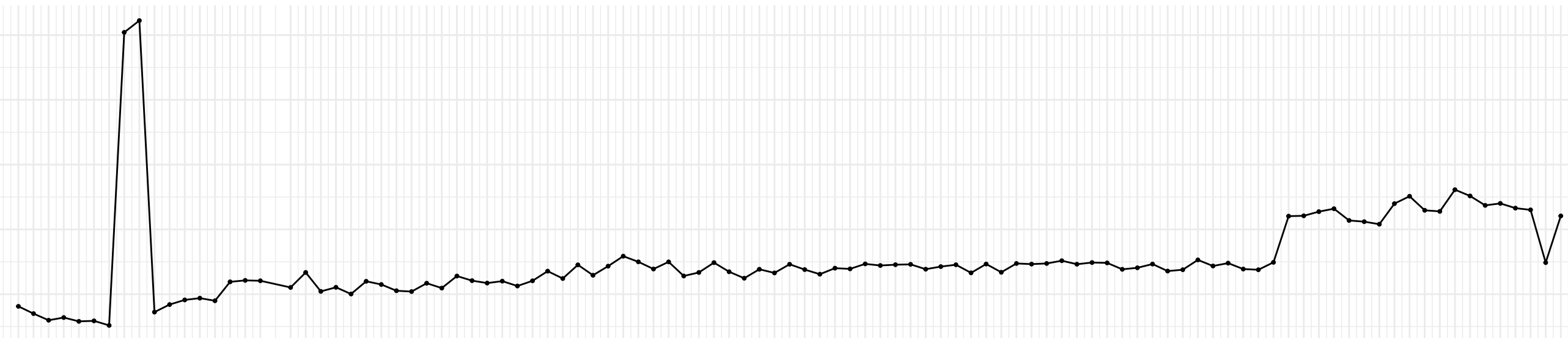
Evolution of TOTRESNS OLS coefficient across time
