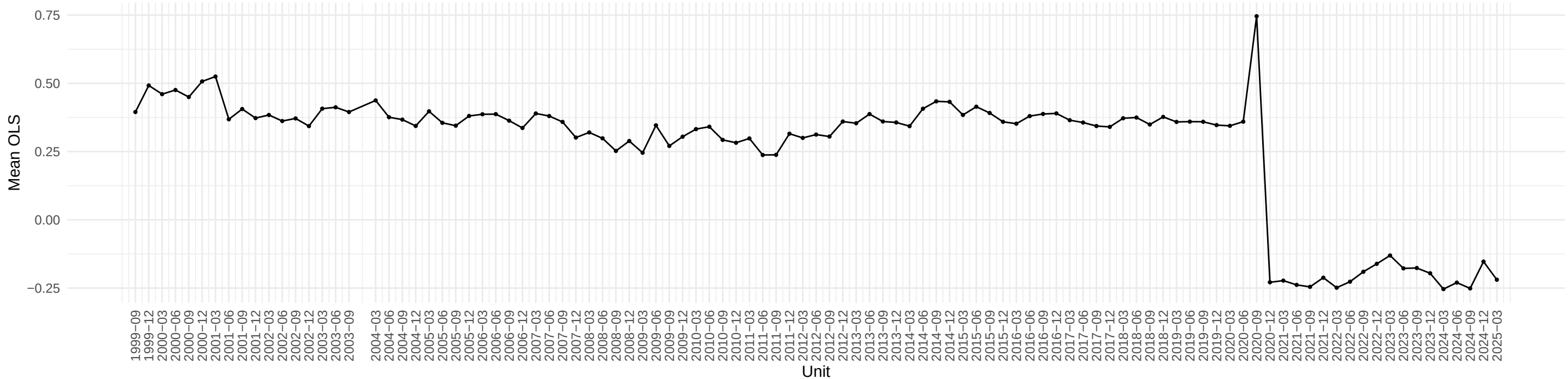
Evolution of UEMP15T26 OLS coefficient across time
