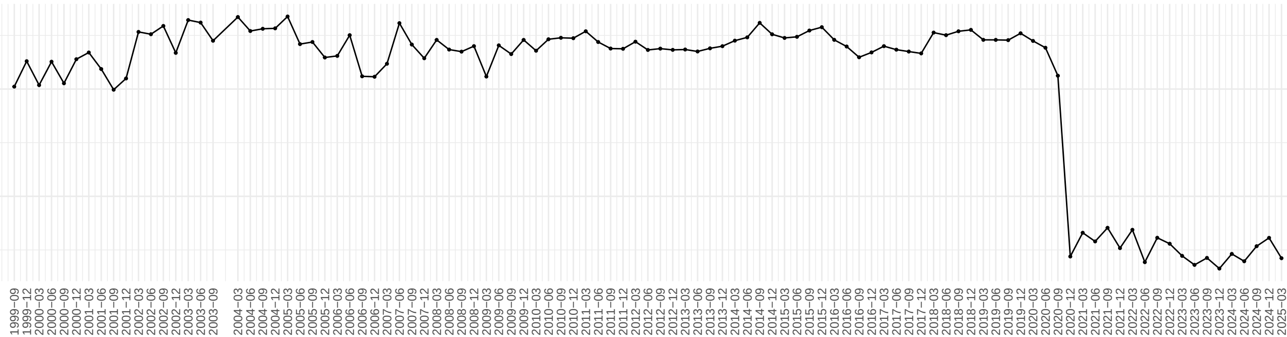
Evolution of UEMP27OV OLS coefficient across time
