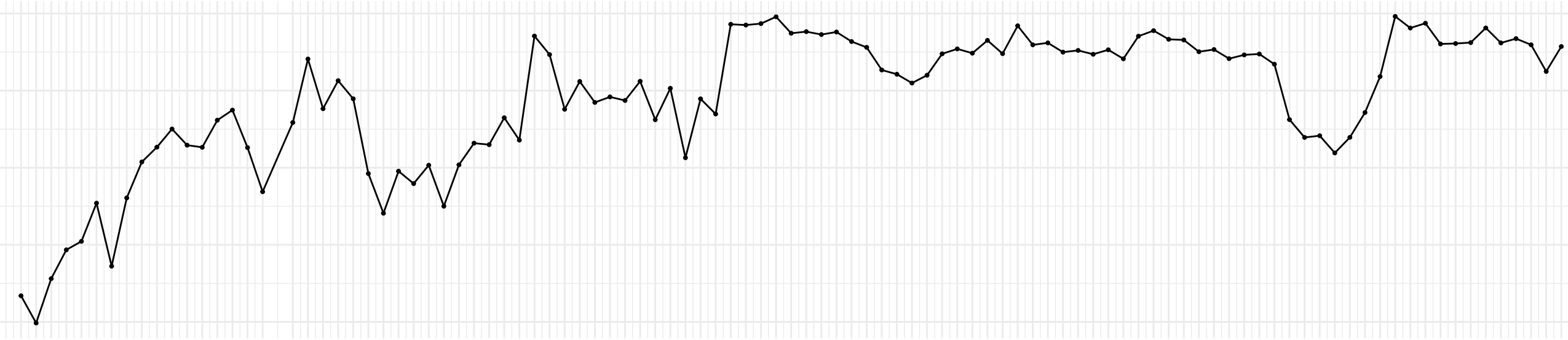
Evolution of UEMPMEAN OLS coefficient across time
