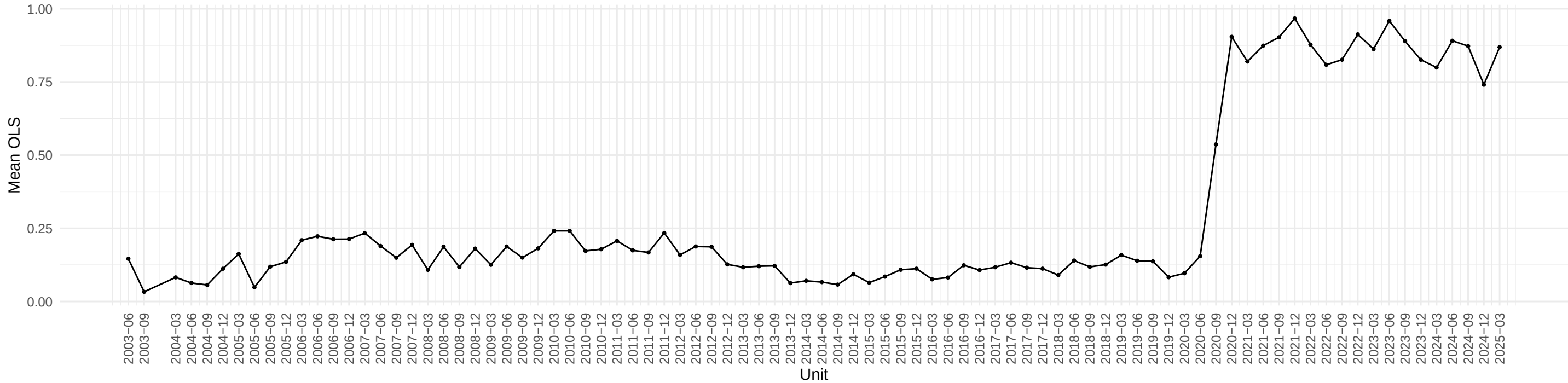
Evolution of USTPU OLS coefficient across time
