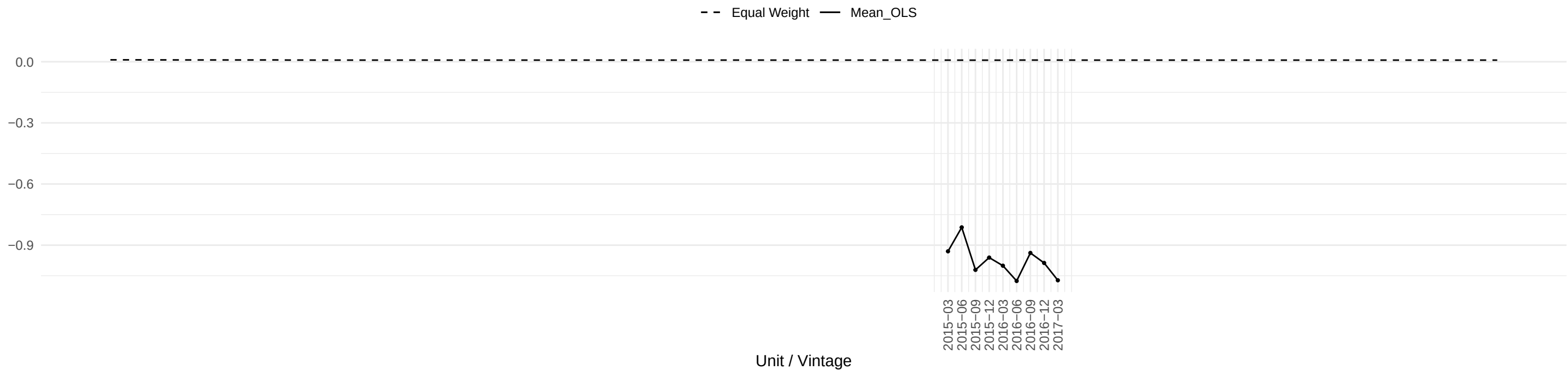
Evolution of CUUR0000SA0L2 OLS coefficient across time
