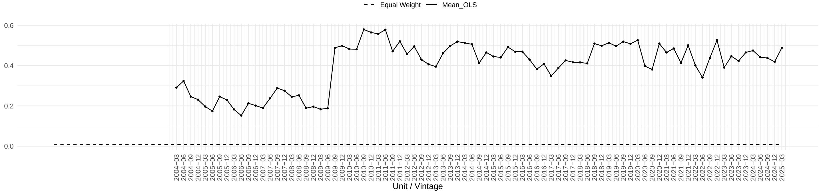
Evolution of DPCERA3M086SBEA OLS coefficient across time
