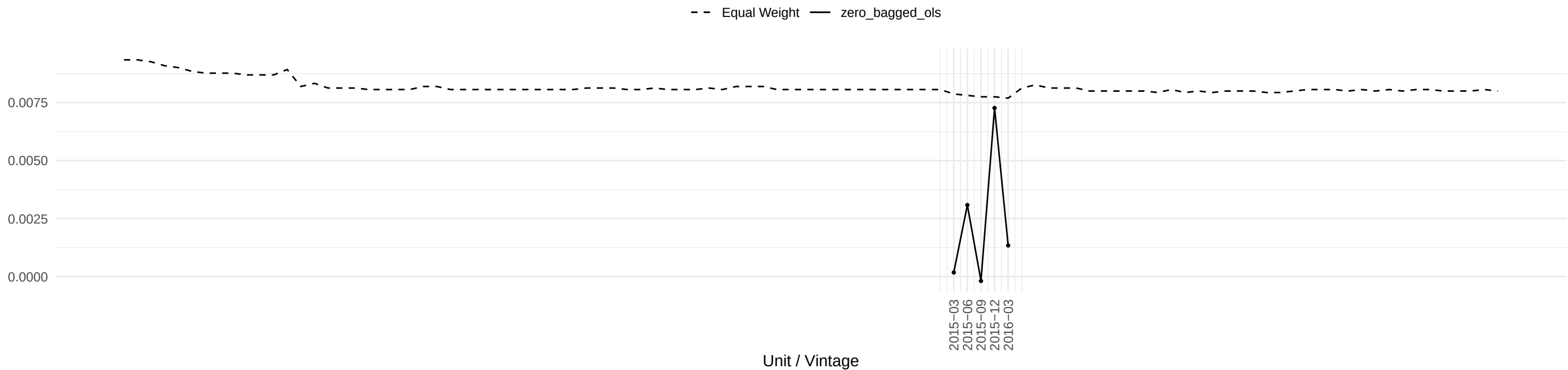
Evolution of NAPMII OLS coefficient across time
