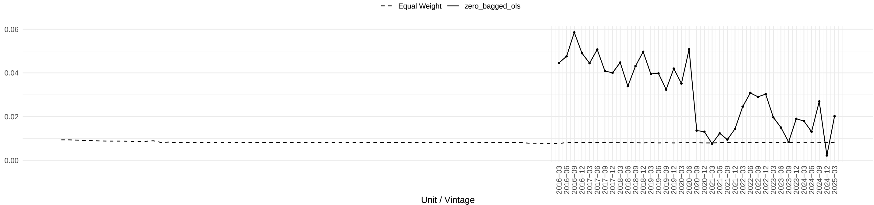
Evolution of WPSID62 OLS coefficient across time
