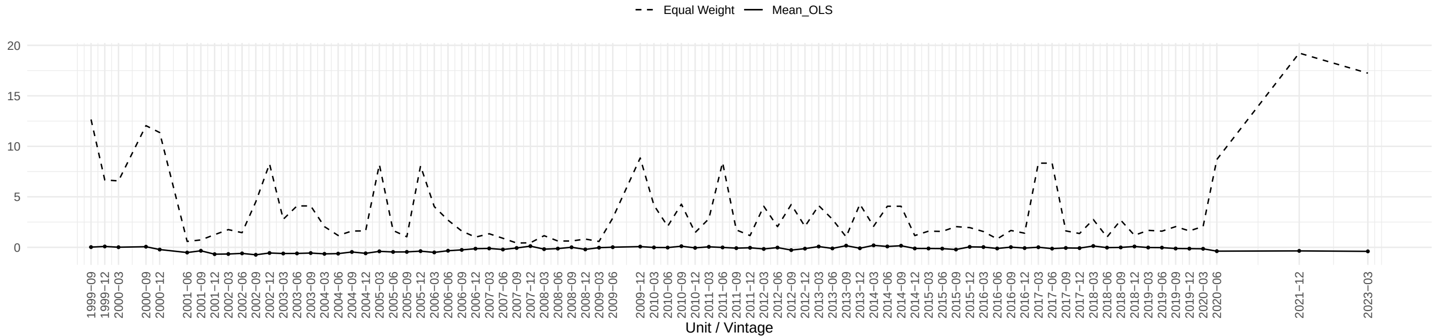
Evolution of T5YFFM OLS coefficient across time
