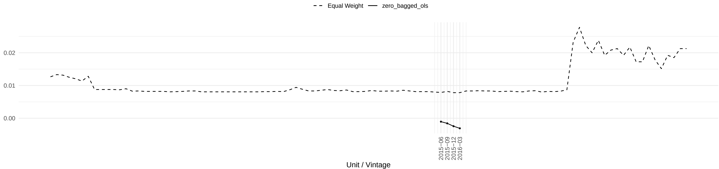
Evolution of NAPMPRI OLS coefficient across time
