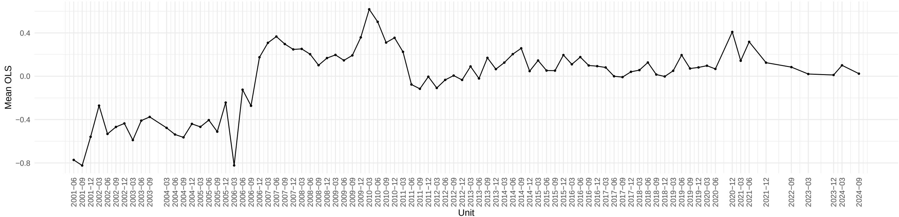
Evolution of ACOGNO OLS coefficient across time
