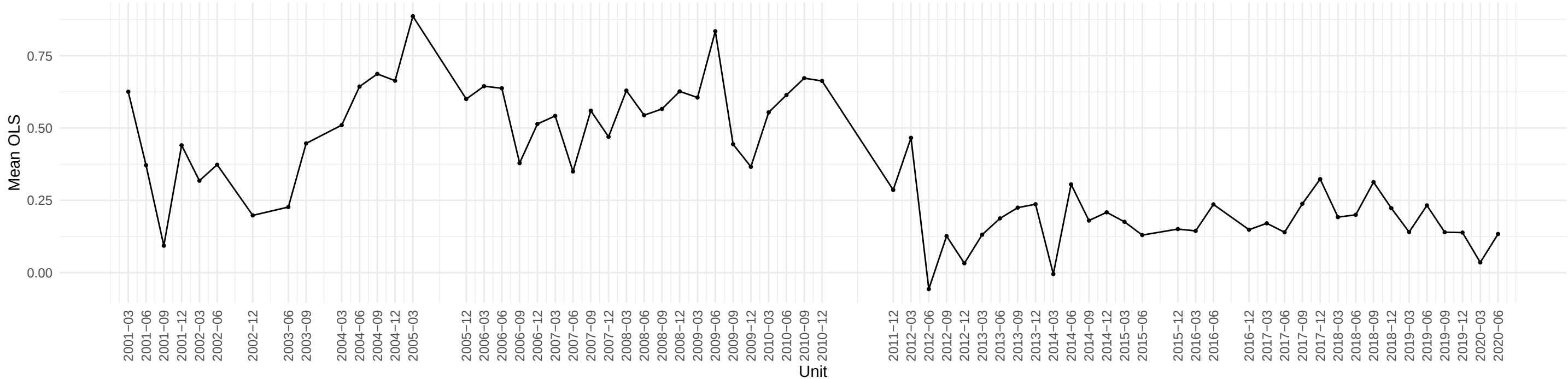
Evolution of DTCOLNVHFM OLS coefficient across time
