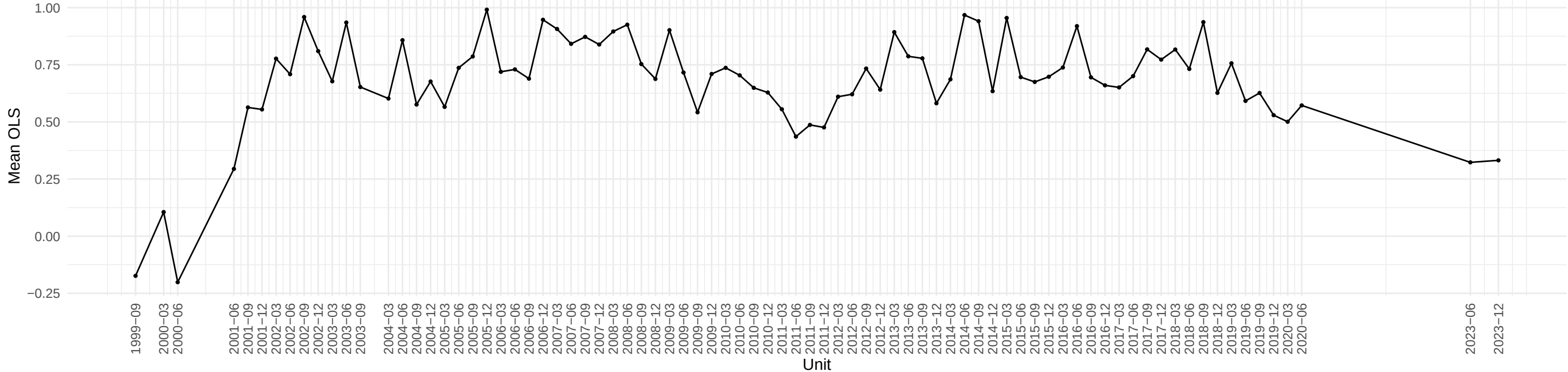
Evolution of GS10 OLS coefficient across time
